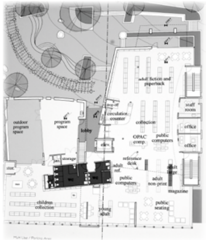
Design plans for the New Salt Spring Island Public Library.
